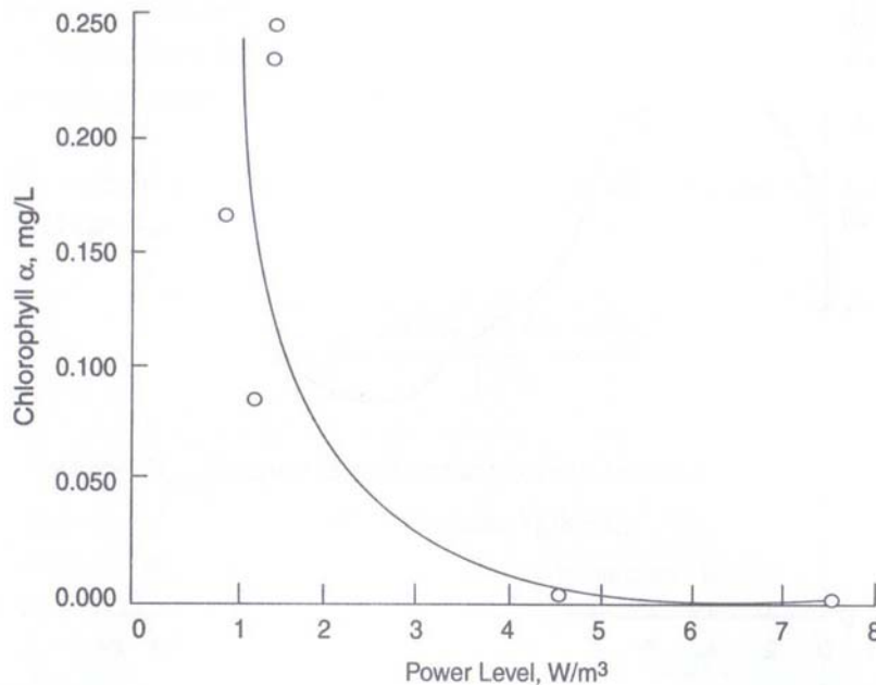
Figure 2. Chlorophyll a concentration in effluents of aerated lagoon basins as a function of aeration power intensity (Source: Rich, 1978)
